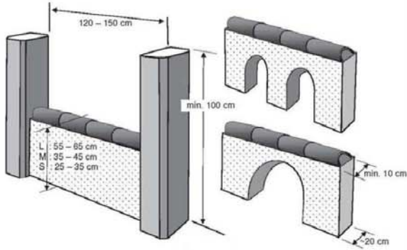
Wall / Viaduct
